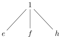
FIGURE 5. Hasse Diagram of S
