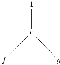
FIGURE 6. Hasse Diagram of S
