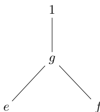
FIGURE 4. Hasse Diagram of S
