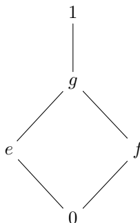
FIGURE 3. Hasse Diagram of S
